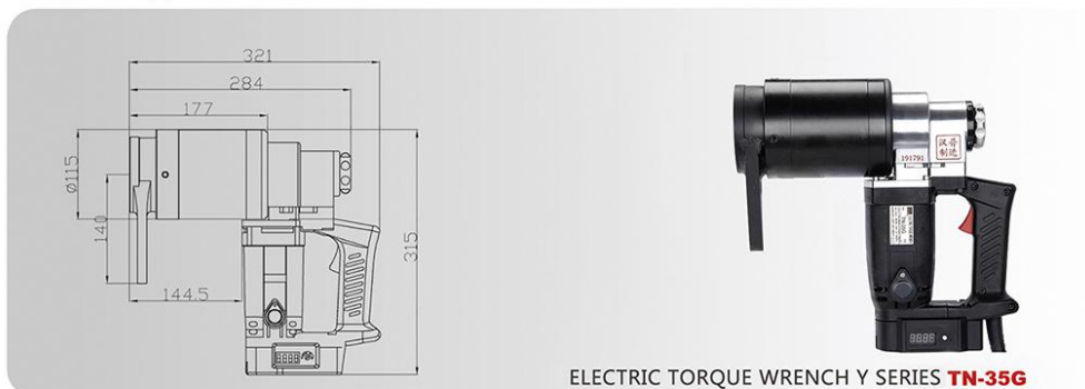
ELECTRIC TORQUE WRENCH Y SERIES TN-35G
